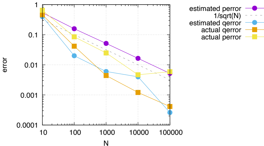
error of the unit circle are using plain MC and quasi-random MC
